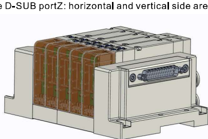
Horizontal plug-in
