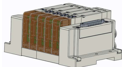
Vertical plug-in
