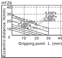
The range of the closed gripping points
