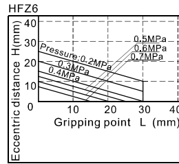
The range of the opened clamping point
