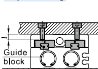
Top Mounting
