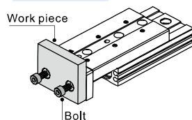
Front Mounting
