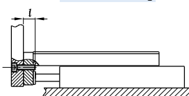
Front Mounting
