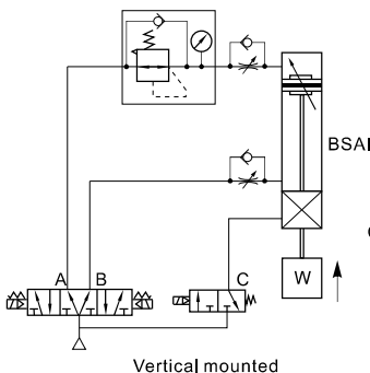
Vertical mounted
