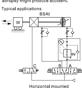
Horizontal mounted
